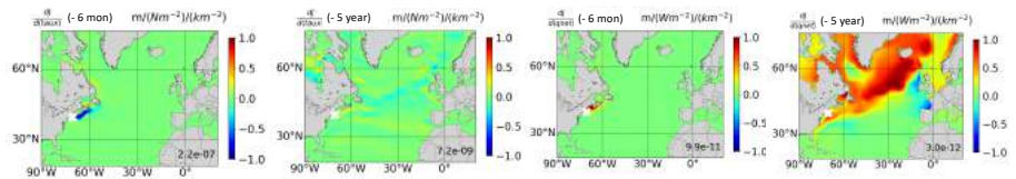
Figure 2. Examples of the sensitivities of Nantucket SL to forcings computed by the ECCO adjoint: response of Nantucket SL to a unit positive perturbation of zonal wind stress at different locations with 6-month (a) and 5-year (b) lead times. (c) & (d) are the equivalent maps for SL response to air-sea heat flux. All maps were normalized by the respective maximum sensitivity value for each lead time (shown in the lower right corner of each panel).
