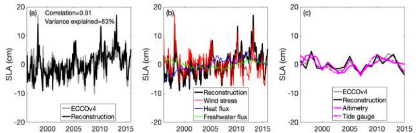
Figure 3. (a) Non-seasonal SLA from ECCOv4 & adjoint reconstruction. (b) Decomposition of reconstructed SLA into contributions by winds & air-sea heat/freshwater fluxes. (c) detrended annually averaged SLA from ECCOv4, reconstruction, altimetry, and tide gauge. Atmospheric pressure effect were removed from ECCOv4, altimetry, and tide gauge data.
