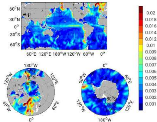
Figure: STD of Total Adjustment ( \text{N/m}^2 ): \tau_v
