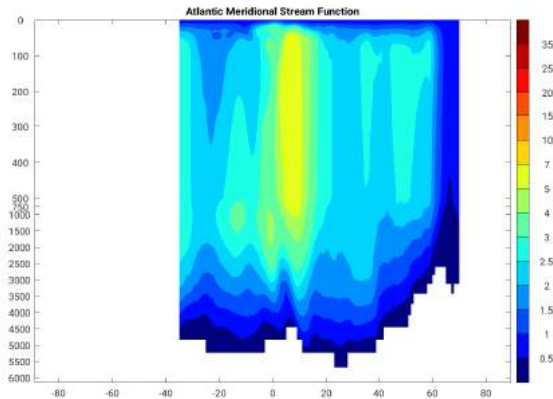
Figure: Atlantic Overturning Streamfunction ( S_v ): Standard Deviation, 1992 thru 2015
