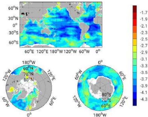
Figure: Sea Level Anomaly, Large Scale: Modeled-Data log(variance) (m 2 )
