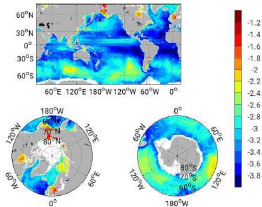
Figure: Sea Level Anomaly, Pointwise: Modeled \log(\text{variance}) ( m^2 )
