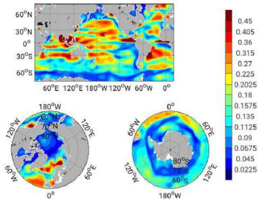
Figure: RMS of Total Adjustment (m/yr): precip
