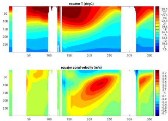
Figure: Equator Temperature (C;top) and Zonal Velocity (m/s;bottom): 1992 thru 2015 Mean
