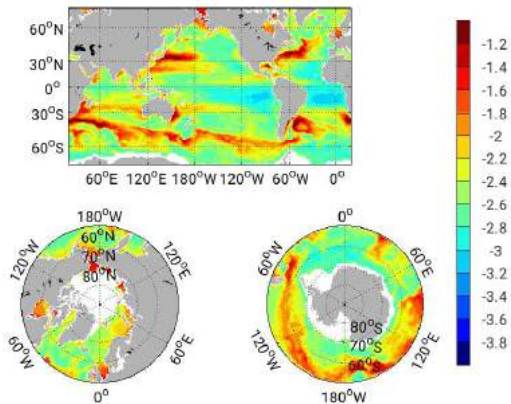
Figure: Sea Level Anomaly, Pointwise: Data log(variance) ( \text{m}^2 )
