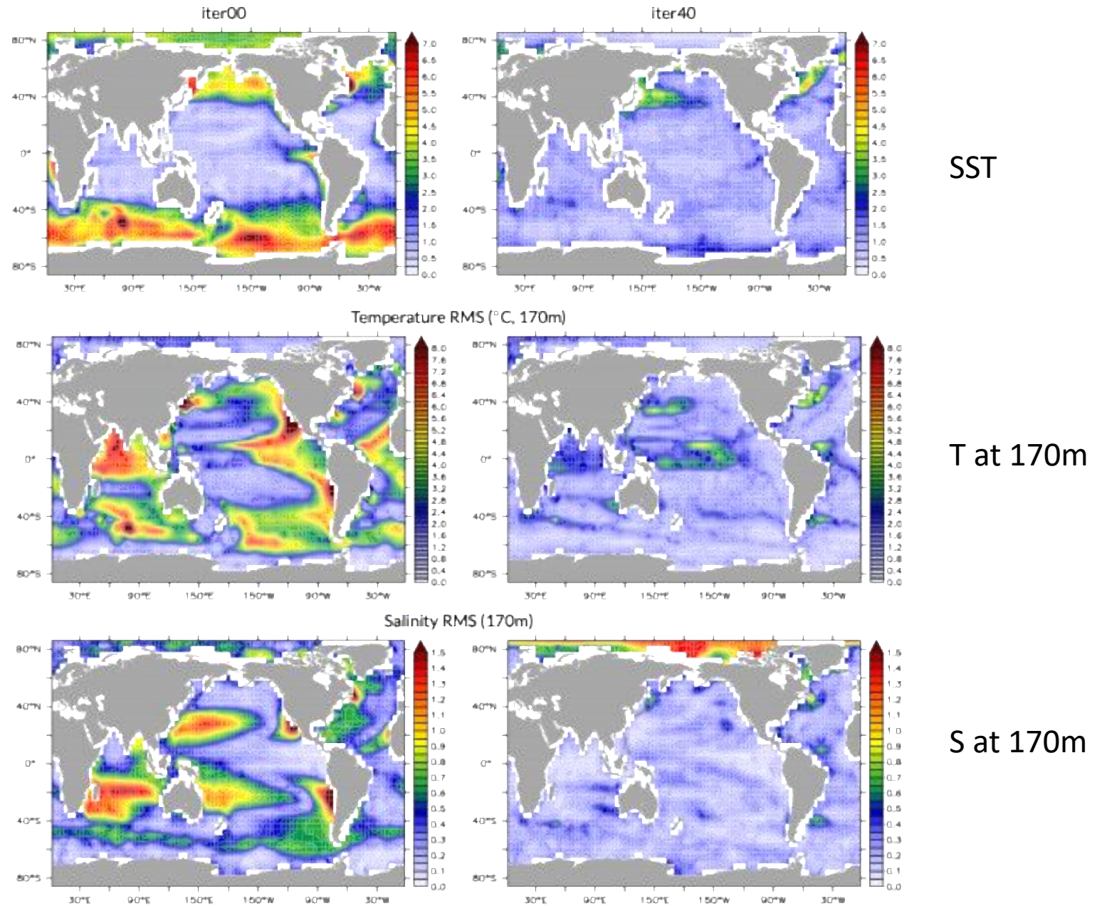
FIGURE 5 RMS difference between simulated temperature and salinity and the EN4 in situ data at 170 m.
